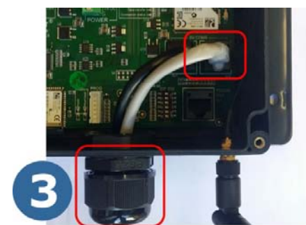
3 Feed existing cable through gland and connect into spare socket labelled RJ3, tighten gland and screw lid back in place
