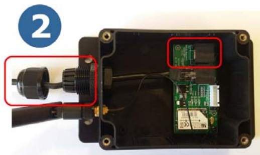
2 Remove lid and cable gland from SpaLINK Module
